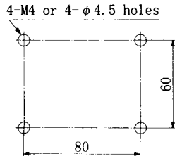
PS5R-C□, D□ Mounting Hole Layout
