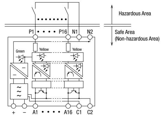
Connector Wiring, Sink Output
